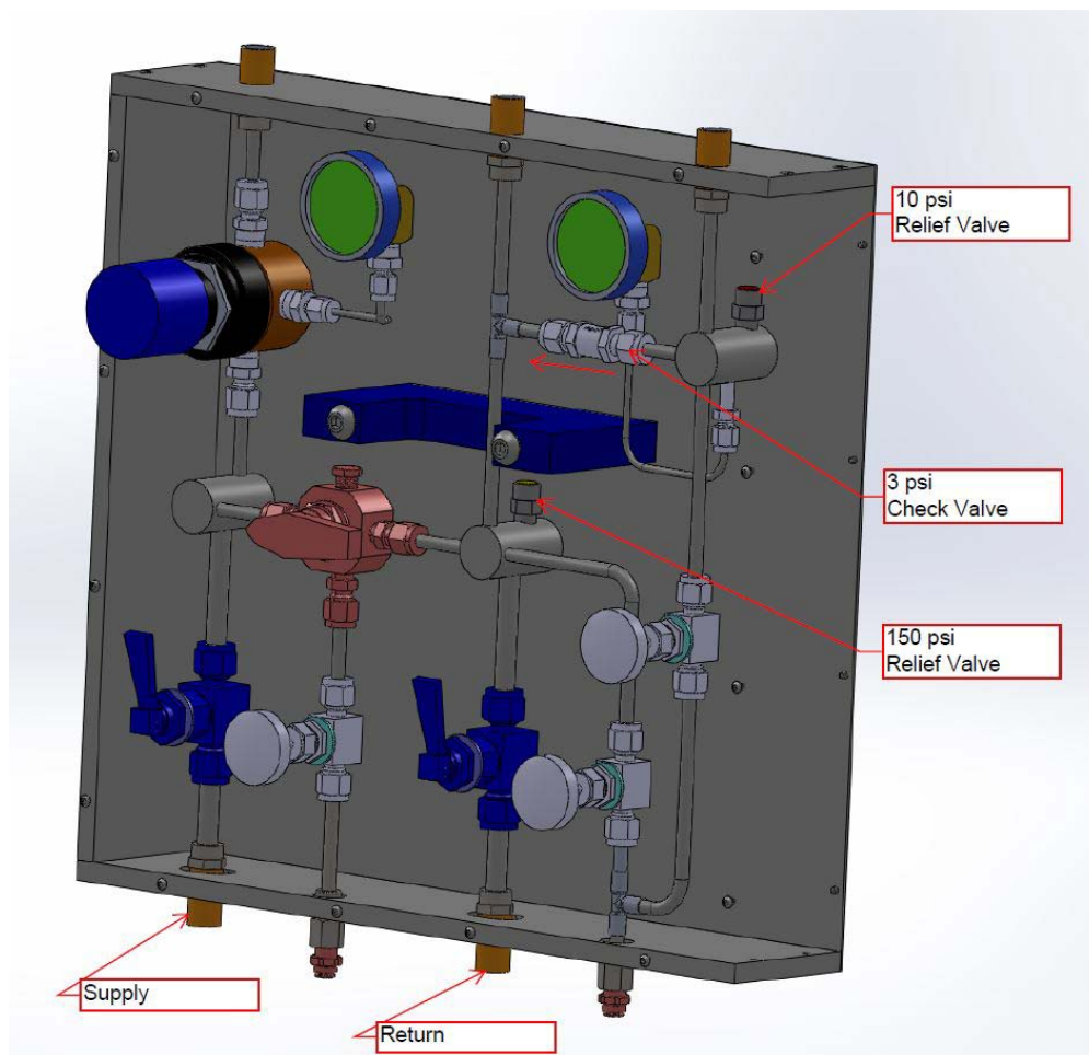
Figure 3-20 Gas Manifold - Interior
